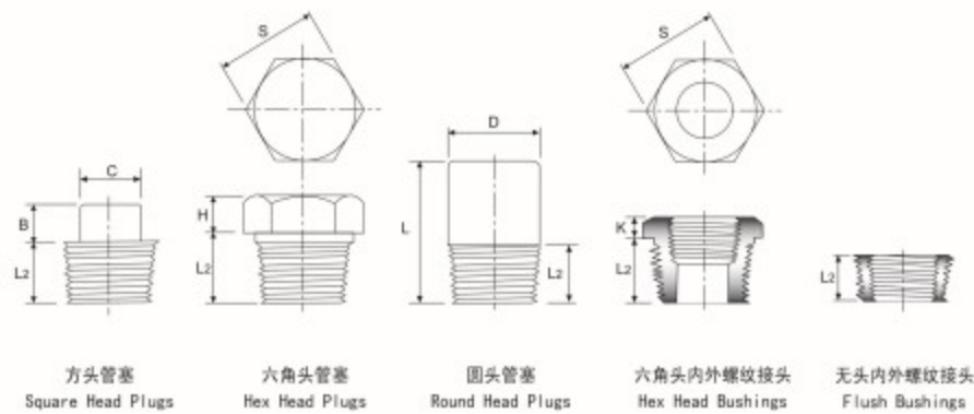
螺纹管件 Threaded Fittings GB/T 14626、ASME B16.11
